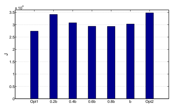
FIG. 7: The values of objective function (3) on the Star network with the optimal pinning control, and different constant pinning controls on the first node with control strengths from 0.2b to b . ‘Opt1’, ‘Opt2’ denote u_1^* and u_2^* , respectively.
