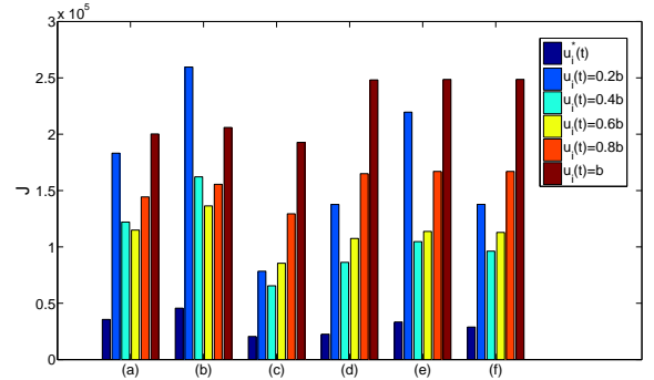
FIG. 3: (Color online) The values of the objective function (3) on different complex networks with different controls. With the parameters (i),(a),(b),(c) are obtained on Star network, Watts-Strogatz network, BA network, respectively; with the parameters (ii),(d),(e),(f) are obtained on Star network, Watts-Strogatz network, BA network, respectively.
