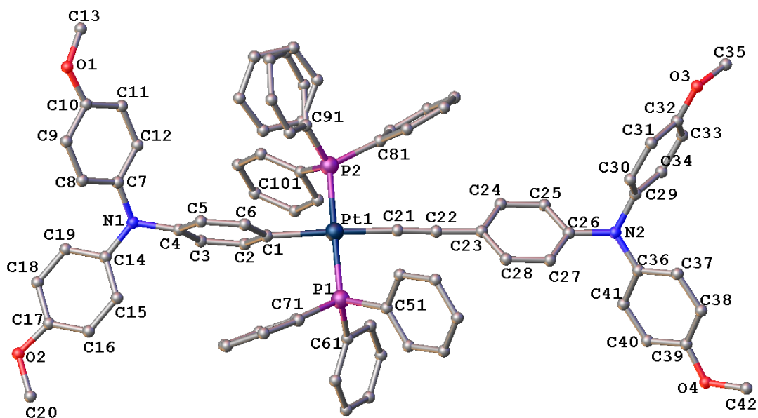
Figure 2. A plot of a molecule of 4b showing the atom labelling scheme, with thermal ellipsoids plotted at 50%. The disorder in the C91 ring is shown (see Experimental), and hydrogen atoms have been omitted for clarity.
