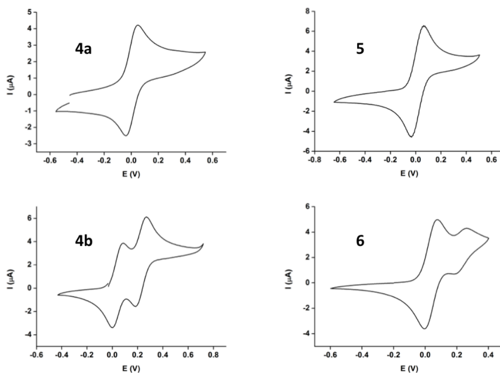
Figure 3. Plots of the cyclic voltammograms of 4a , 4b , 5 and 6 in \text{CH}_2\text{Cl}_2 with 0.1 M \text{NBu}_4[\text{PF}_6] at a scan rate of 100 mV/s and referenced against [\text{FeCp}^*_2/\text{FeCp}^*_2]^+ at -0.48 V vs \text{FeCp}_2 / [\text{FeCp}_2]^+ = +0.0 V.
