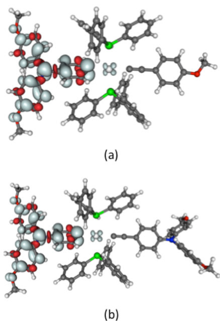
Figure 7. Plots of the spin density in (a) [4a] + and (b) [4b] +
