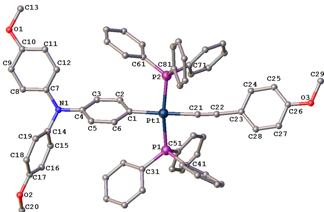
Figure 1. A plot of a molecule of 4a showing the atom labelling scheme, with thermal ellipsoids plotted at 50%. Hydrogen atoms have been omitted for clarity.
