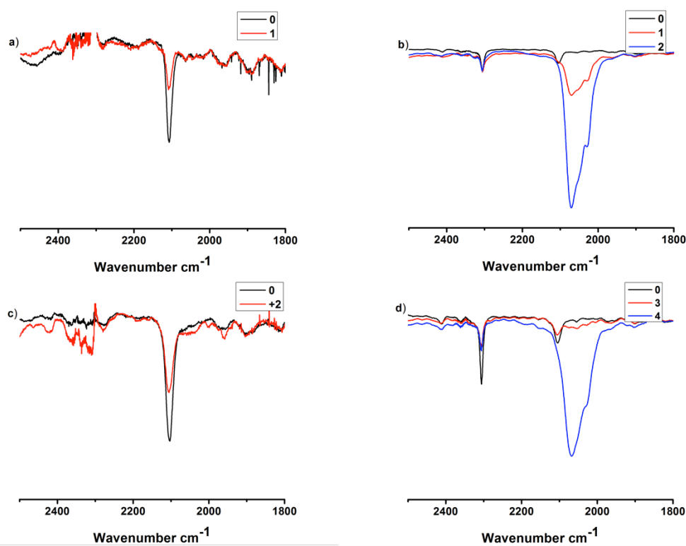
Figure 4: IR spectra of (a) [4a] n+ , (b) [4b] n+ , (c) [5] n+ and (d) [6] n+ showing the \nu(\text{C}\equiv\text{C}) band in the various oxidation states generated by in situ electrochemical oxidation in CH 2 Cl 2 / 0.1 M NBu 4 PF 6 in an OTTLE cell
