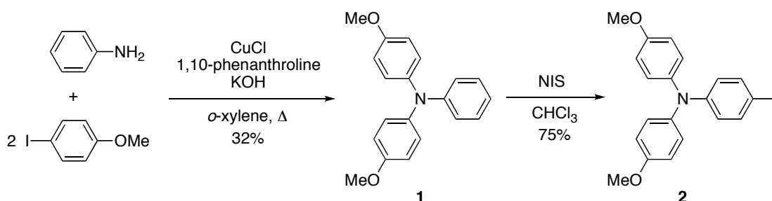
Scheme 1. The preparation of 1 and 2
