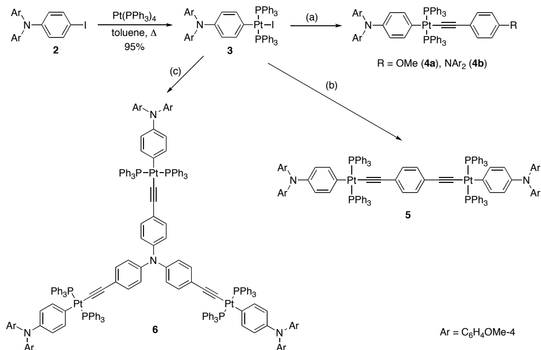
Scheme 2. The preparation of 3 , 4a , 4b , 5 and 6 . (a) CuI (cat) / NHEt 2 / HC≡CC 6 H 4 R. (b) CuI (cat) / NHEt 2 / HC≡CC 6 H 4 C≡CH. (c) CuI (cat) / NHEt 2 / N(C 6 H 4 C≡CH-4) 3 .
