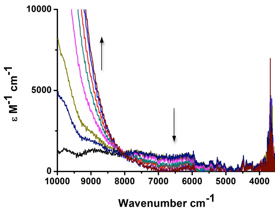
Figure 5. An expansion of the NIR region of [\mathbf{4b}]^+ on oxidation to [\mathbf{4b}]^{2+} showing the collapse of the IVCT band
