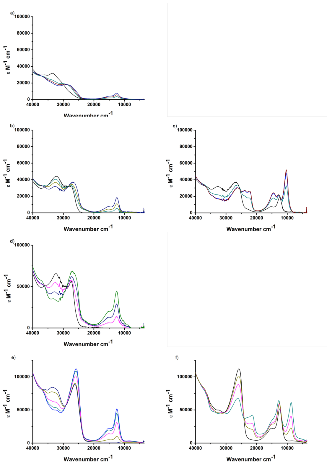
Figure 6: UV-vis-NIR spectra of (a) [4a] \rightarrow [4a]^+ , (b) [4b] \rightarrow [4b]^+ , (c) [4b]^+ \rightarrow [4b]^{2+} , (d) [5] \rightarrow [5]^{2+} , (e) [6] \rightarrow [6]^{3+} and (f) [6]^{3+} \rightarrow [6]^{4+} showing the changes in the various oxidation states generated by in situ electrochemical oxidation in \text{CH}_2\text{Cl}_2 / 0.1 \text{ M NBu}_4\text{PF}_6 in an OTTLE cell.
