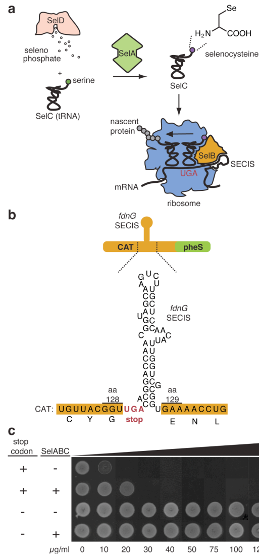
Figure 1. A selection system to analyze selenocysteine incorporation in E. coli . (a) The process of selenocysteine incorporation in prokaryotes. (b) Schematic representation of the reporter mRNA showing the sequence and location of the E. coli fdnG SECIS. (c) Chloramphenicol (Cm) resistance derived from a SECIS-containing reporter depends on the overexpression of SelA, SelB and SelC.
