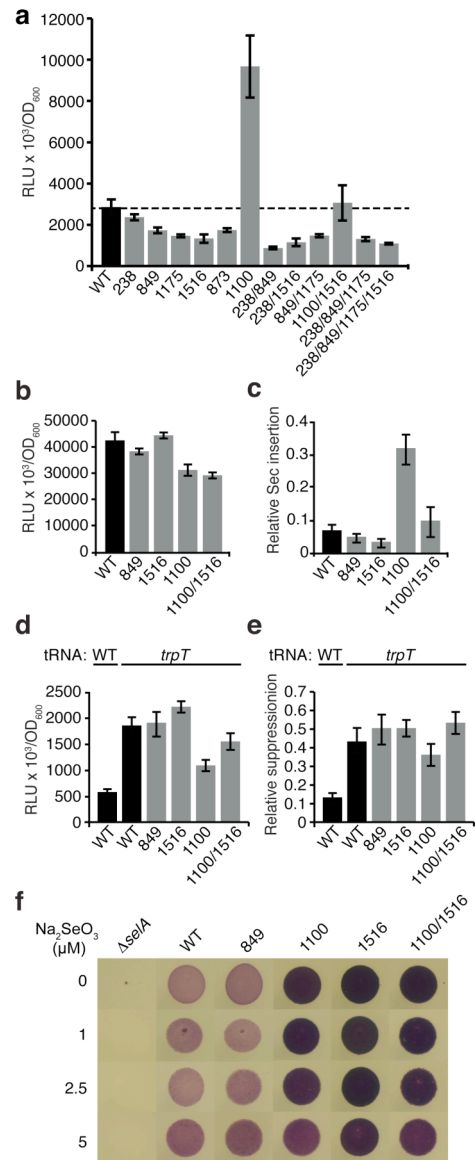
Figure 3. Mutant ribosomes with impaired or enhanced selenocysteine incorporation, independent of canonical UGA suppression. (a) The efficiency of selenocysteine incorporation by mutant ribosomes. Mutant and wild-type ribosomes were expressed as the sole ribosomes in cells deleted for all seven ribosomal operons and expressing a reporter mRNA with the Gaussia princeps luciferase ( GLuc ) located downstream of the fdnG SECIS. Selenocysteine incorporation was determined by measuring luciferase activity, normalized to OD 600 . Clone 1 corresponds to mutant 238/849/1175/1516. (b) The activity of selected ribosomes in canonical translation was determined using a reporter mRNA without a SECIS. (c) The efficiency of selenocysteine incorporation by mutant ribosomes, normalized to canonical translation. (d) The effect of 16S rRNA mutations on tryptophan-mediated suppression by tRNA Trp(UCA) . Overexpressed wild-type tRNA Trp(CCA) (WT) was used as a control. (e) tRNA Trp(UCA) (TrpT)-mediated suppression, normalized to canonical translation. (f) Selenocysteine incorporation into endogenous formate dehydrogenase is affected by mutations in 16S rRNA, determined by the reduction of benzyl viologen. 3
