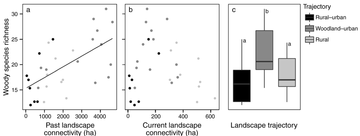
FIG. 3. Relationship between richness of woody species and (a) historical connectivity ( r = 0.62 , P < 0.001 ), (b) current connectivity ( r = -0.10 , P = 0.61 ), and (c) landscape trajectory ( P = 0.023 ; 95% CI). Landscape trajectory is represented as: rural-urban (black), woodland-urban (dark gray), rural (light gray).
