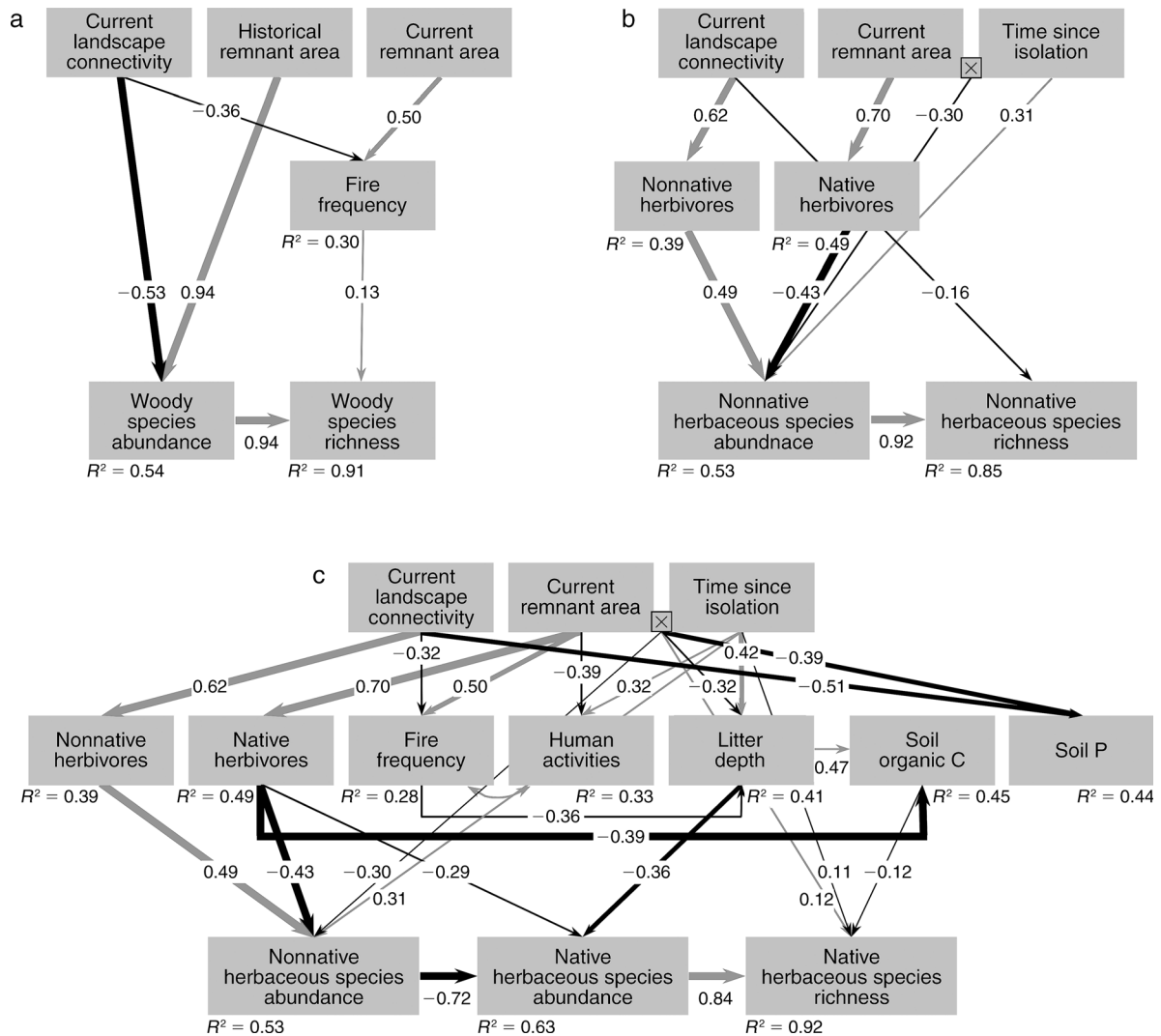
FIG. 4. Best-fitting structural equation models examining the effects of landscape and local factors on the richness and abundance of the (a) woody species ( df = 12 , \chi^2 = 14.34 , P = 0.28 ), (b) nonnative herbaceous species ( df = 14 , \chi^2 = 18.26 , P = 0.19 ), and (c) native herbaceous species ( df = 60 , \chi^2 = 59.68 , P = 0.49 ). Straight single-headed arrows represent significant effects, whereas curved, double-headed arrows represent significant correlations. Gray arrows represent positive effects and black arrows represent negative effects. (c) All the significant paths between landscape and local factors are represented in the model. In the remaining models, only significant effects on the plant community are shown. The strength of each path is given by the arrow thickness, which is proportional to the P values (wider, P \leq 0.001 ; intermediate, P \leq 0.01 ; narrower, P \leq 0.05 ), and the standardized coefficients.
