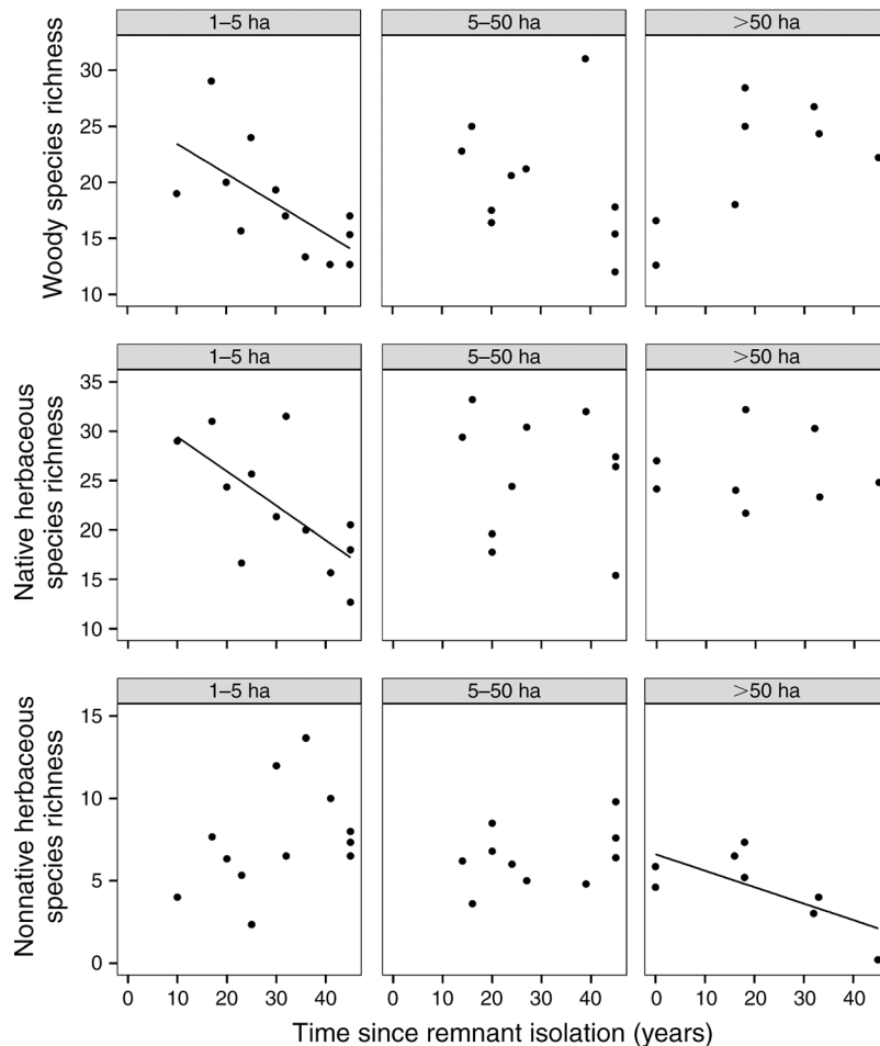
FIG. 2. Relationship between richness of (top) woody species, (middle) native herbaceous species, and (bottom) nonnative herbaceous species with time since isolation, for the three classes of remnant area considered in the study design. The solid circles represent sampled remnants, and the solid regression lines represent significant relationships ( P \leq 0.05 ).
