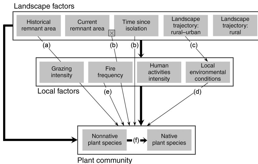
FIG. 1. Conceptual model used in the study. The boxes represent major conceptual constructs. The multiplication symbol ( \times ) between current remnant area and time since isolation represents the interaction term between these variables. Thick arrows represent the general relationships that were examined. Narrow arrows represent the specific relationships that were hypothesized a priori (letters a–f).
