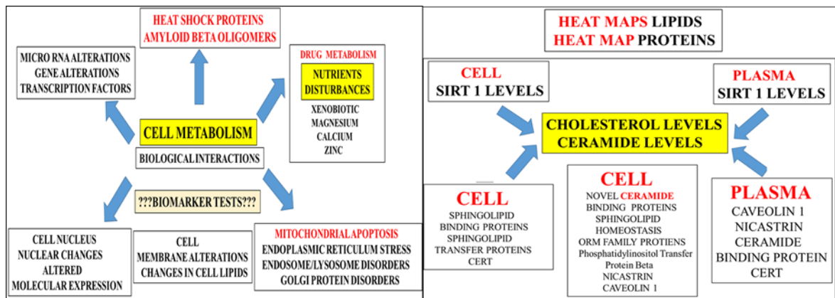
Figure 3: Biomarker tests for mitophagy and ER stress in neuropsychiatric disorders were required for reversal and stabilization of the disease. Genomic, proteomic and lipidomic experiments are critical to assess the induction of mitophagy with relevance Sirt 1 and lipid binding protein analysis in plasma and tissues. Plasma lipid measurements of cholesterol, ceramide, sphingolipids, and phospholipids (phosphatidylinositol) are essential to determine early mitophagy-ER stress disorders in neuropsychiatric disorders.
