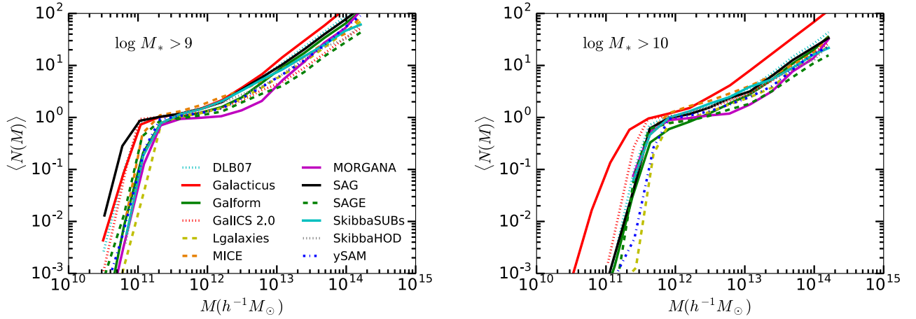
Figure 2. Mean halo occupation number as a function of halo mass for the different models using all the galaxy types. Left-hand panel shows galaxies with M_* > 10^9 h^{-1} M_{\odot} , while the right-hand panel shows galaxies with M_* > 10^{10} h^{-1} M_{\odot} .
